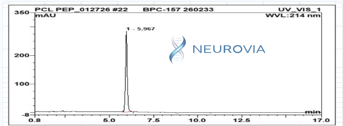
HPLC Chromatogram (Retention Time: _____, 5.967 min)
