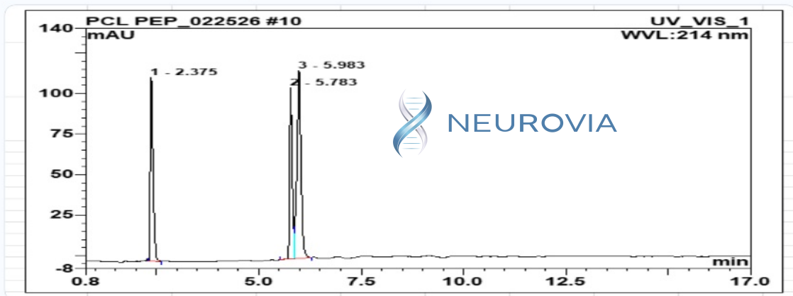
HPLC Chromatogram (Retention Time: 2.375, 5.783, 5.983 min)
