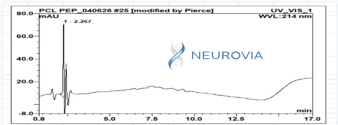
HPLC Chromatogram (Retention Time: 2.267 min)
