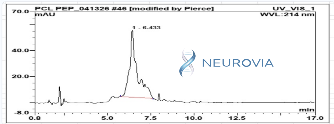
HPLC Chromatogram (Retention Time: 6.433 min)
