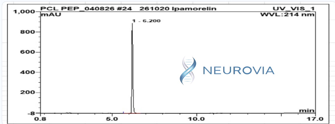
HPLC Chromatogram (Retention Time: 6.200 min)
