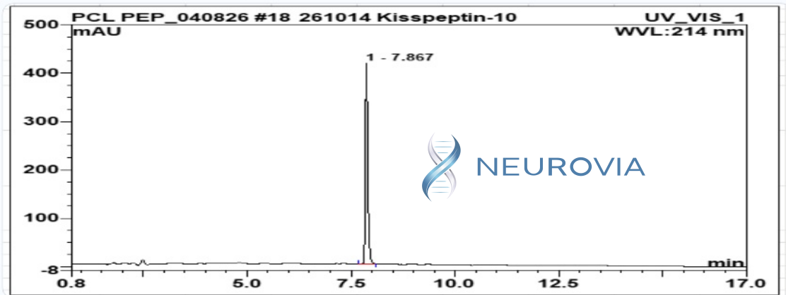
HPLC Chromatogram (Retention Time: 7.867 min)
